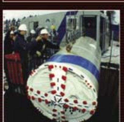
Bottom: Superintendent Bob Welch and crew start slurry micro-tunneling using Ackerman MTBM. New Hampshire.
